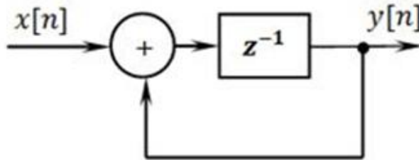
Figure 1. Single-pole filter structure [19] in feedforward path.
