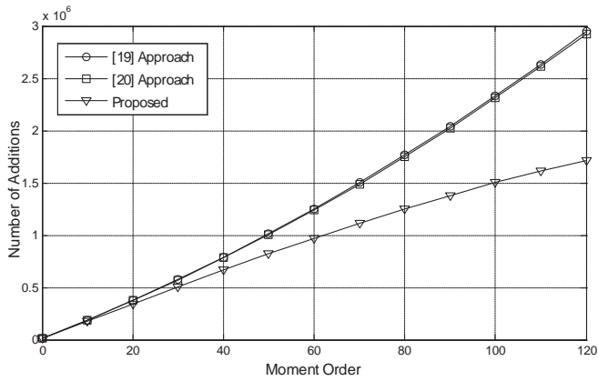
Figure 4. Number of additions for a 128x128 grey-scaled image.
